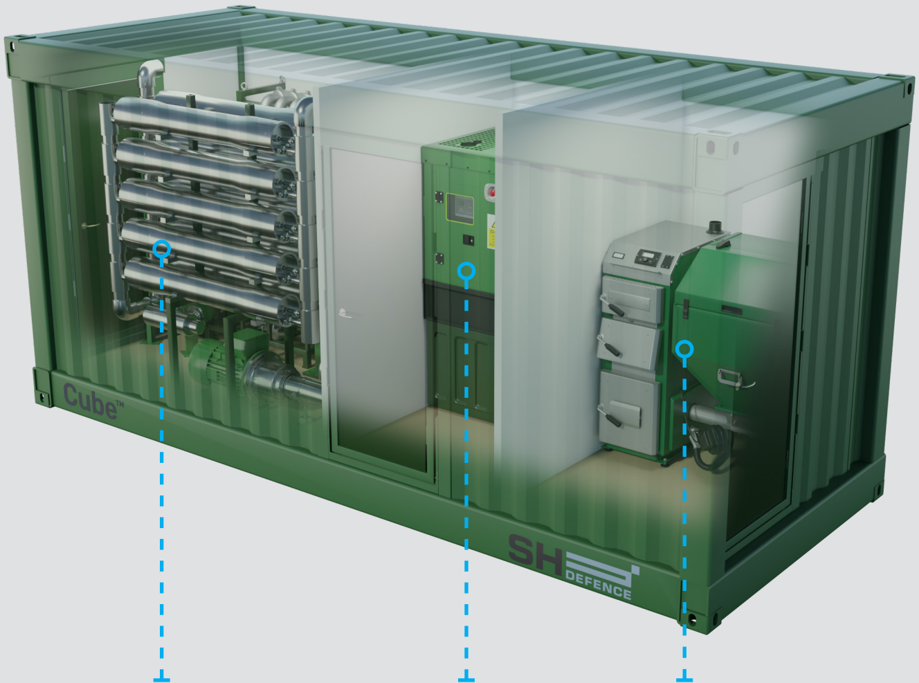
Water treatment system
