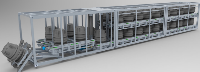
Large setup: 3 x 20' 1x launch 20' and 2x storage 20' (Total-length 18.200 mm)
