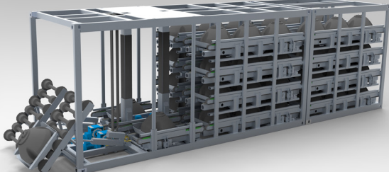
Short setup: 1 x 20' and 1 x 10' 1x launch combi 20' and 1x storage 10' (Total-length 9.100 mm)
